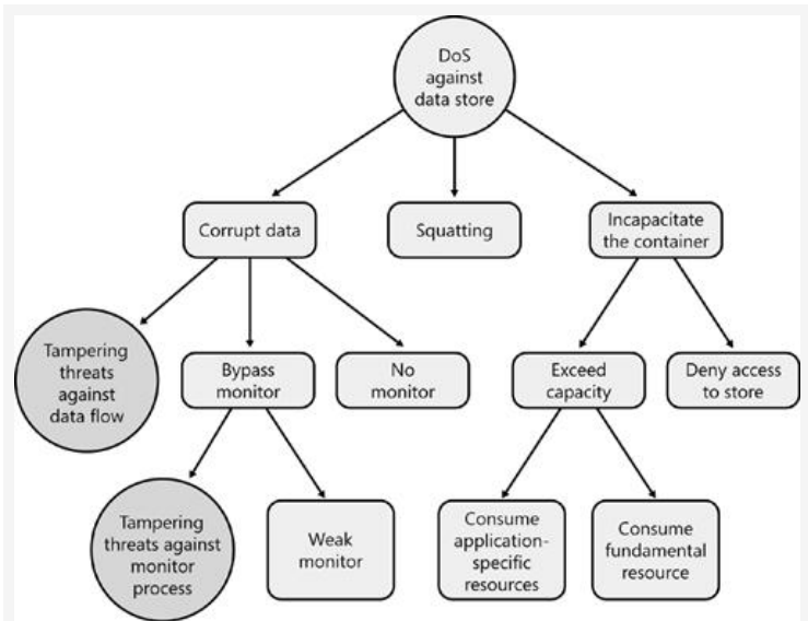
Figure 22-11. Threat tree for denial of service against a data store.
