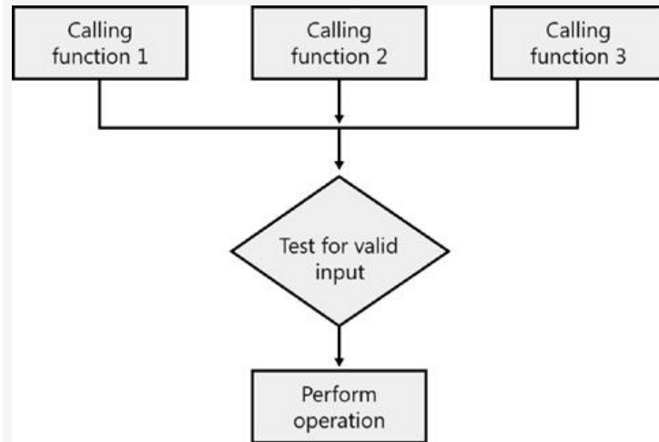
Figure 15-3. Correct fix for an underlying vulnerability.
