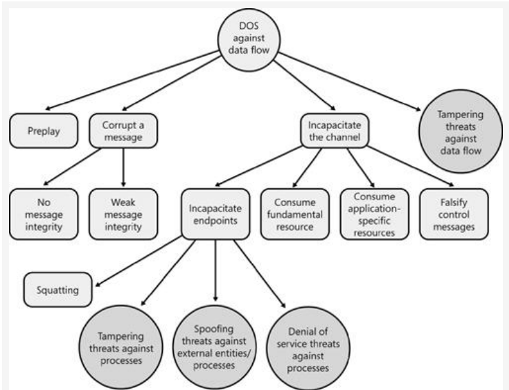
Figure 22-10. Threat tree for denial of service against a data flow.
