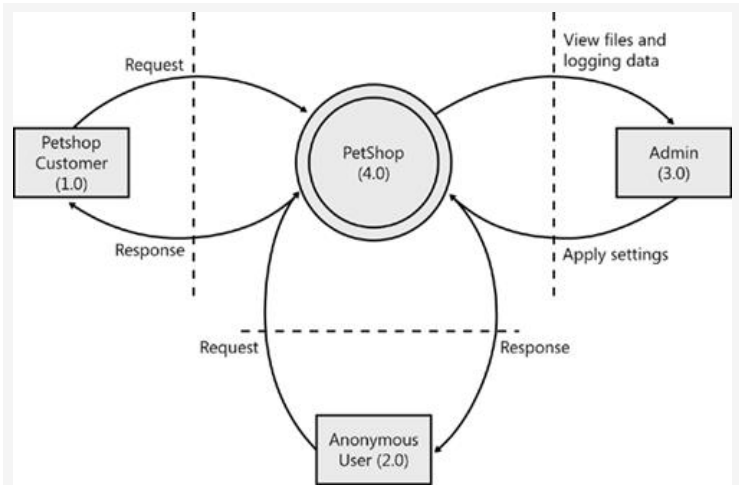
Figure 9-3. Context diagram for Pet Shop 4.0.
