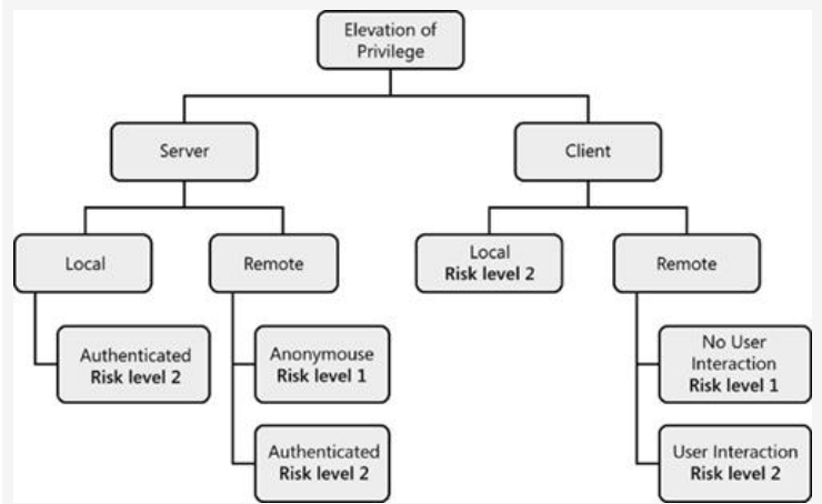
Figure 9-10. EoP threats risk ranking.
