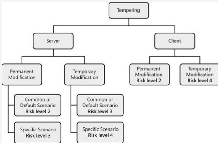
Figure 9-7. Tampering threats risk ranking.
