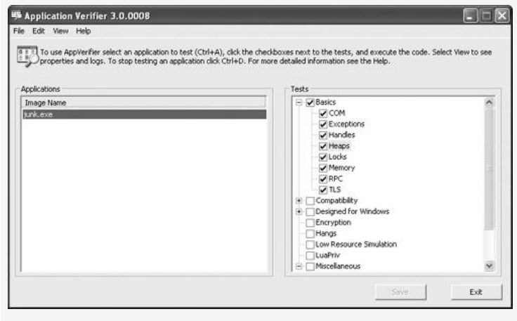
Figure 21-3. AppVerif configuration options in Visual Studio 2005.
