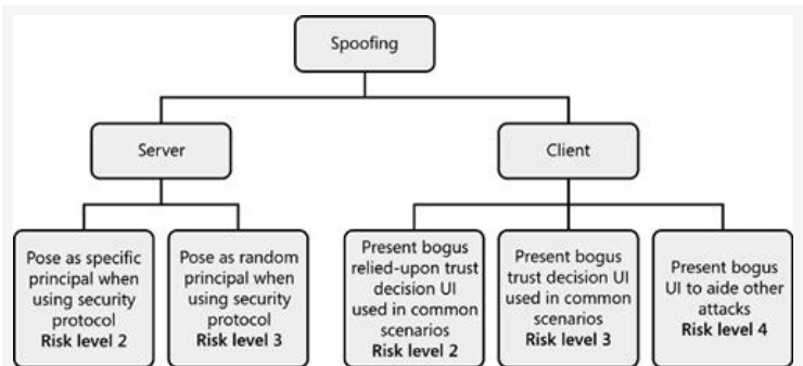
Figure 9-6. Spoofing threats risk ranking.
