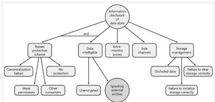
Figure 22-8. Threat tree for information disclosure of a data store.
