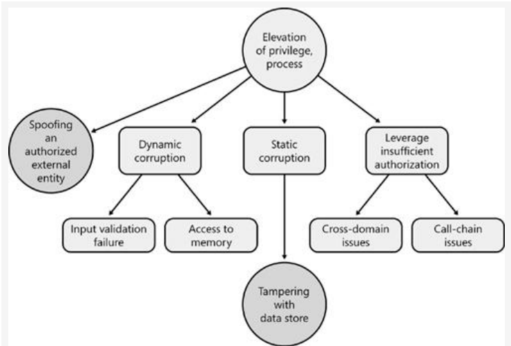
Figure 22-12. Threat tree for elevation of privilege.
