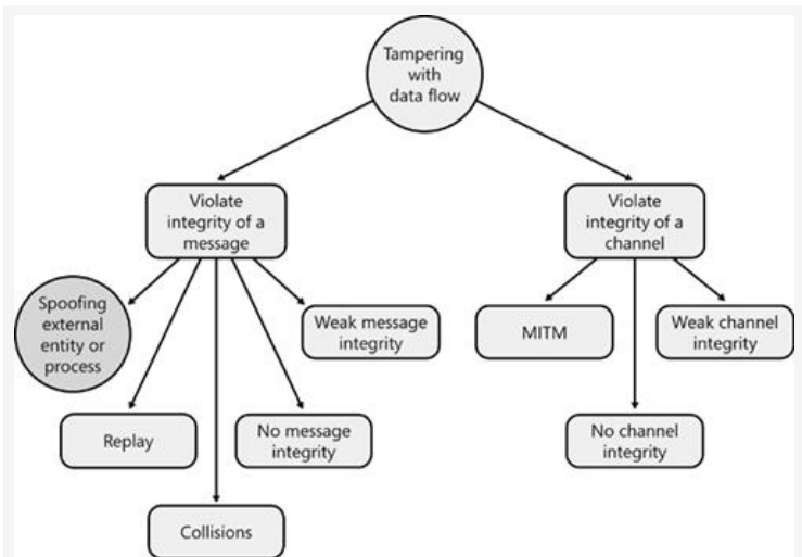
Figure 22-3. Threat tree for tampering with a data flow.
