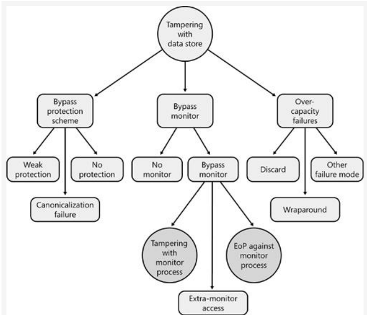
Figure 22-4. Threat tree for tampering with a data store.
