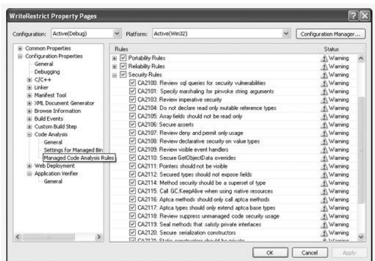
Figure 21-2. Setting managed-code FxCop code-analysis options within Visual Studio 2005.
