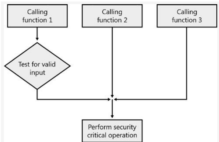
Figure 15-2. Partial fix for an underlying vulnerability.
