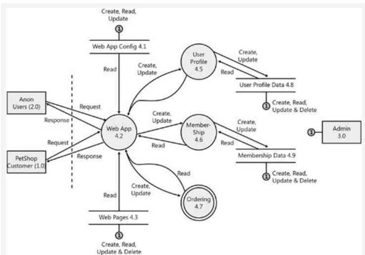
Figure 9-4. The level-0 DFD for Pet Shop 4.0.
