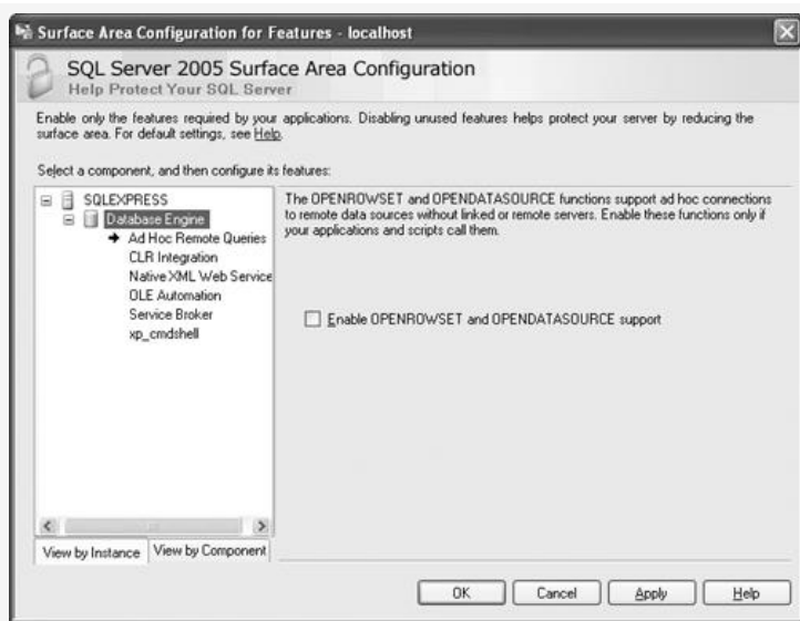
Figure 7-4. SQL Server 2005 can reduce features.
