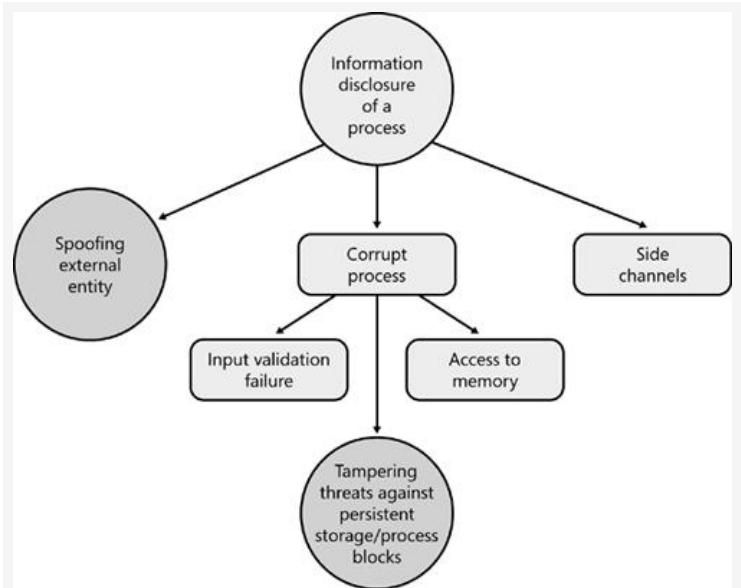
Figure 22-6. Threat tree for information disclosure of a process.
