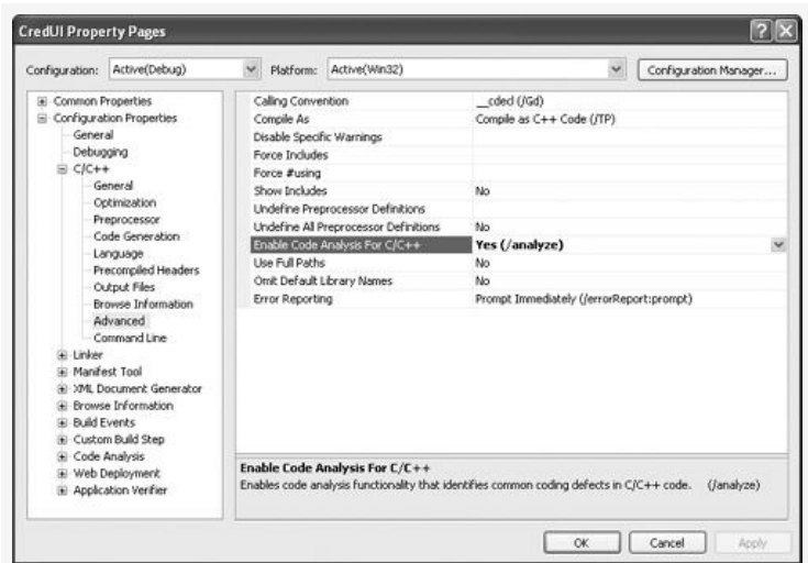
Figure 21-1. Setting the /analyze option in Visual Studio 2005.
