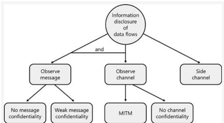
Figure 22-7. Threat tree information disclosure of a data flow.
