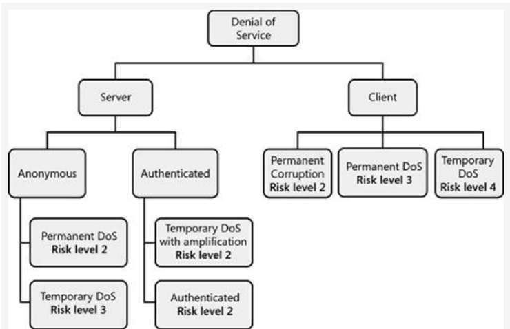
Figure 9-9. DoS threats risk ranking.
