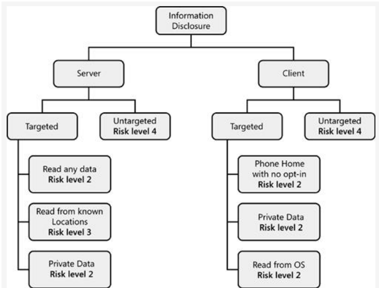
Figure 9-8. Information disclosure threats risk ranking.
