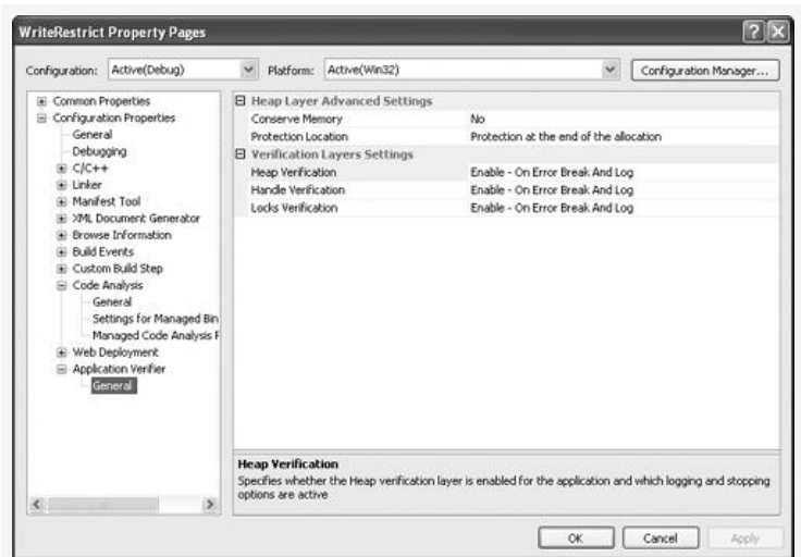
Figure 21-3. AppVerif configuration options in Visual Studio 2005.
