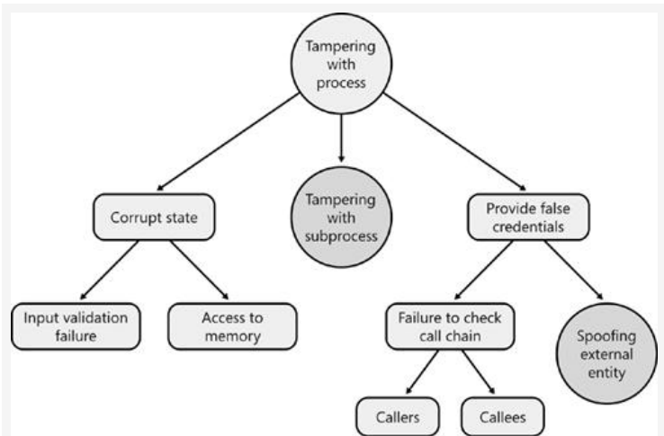
Figure 22-2. Threat tree for tampering with a process.
