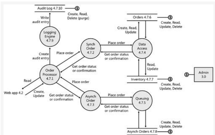
Figure 9-5. The level-1 DFD for order processing within Pet Shop 4.0.
